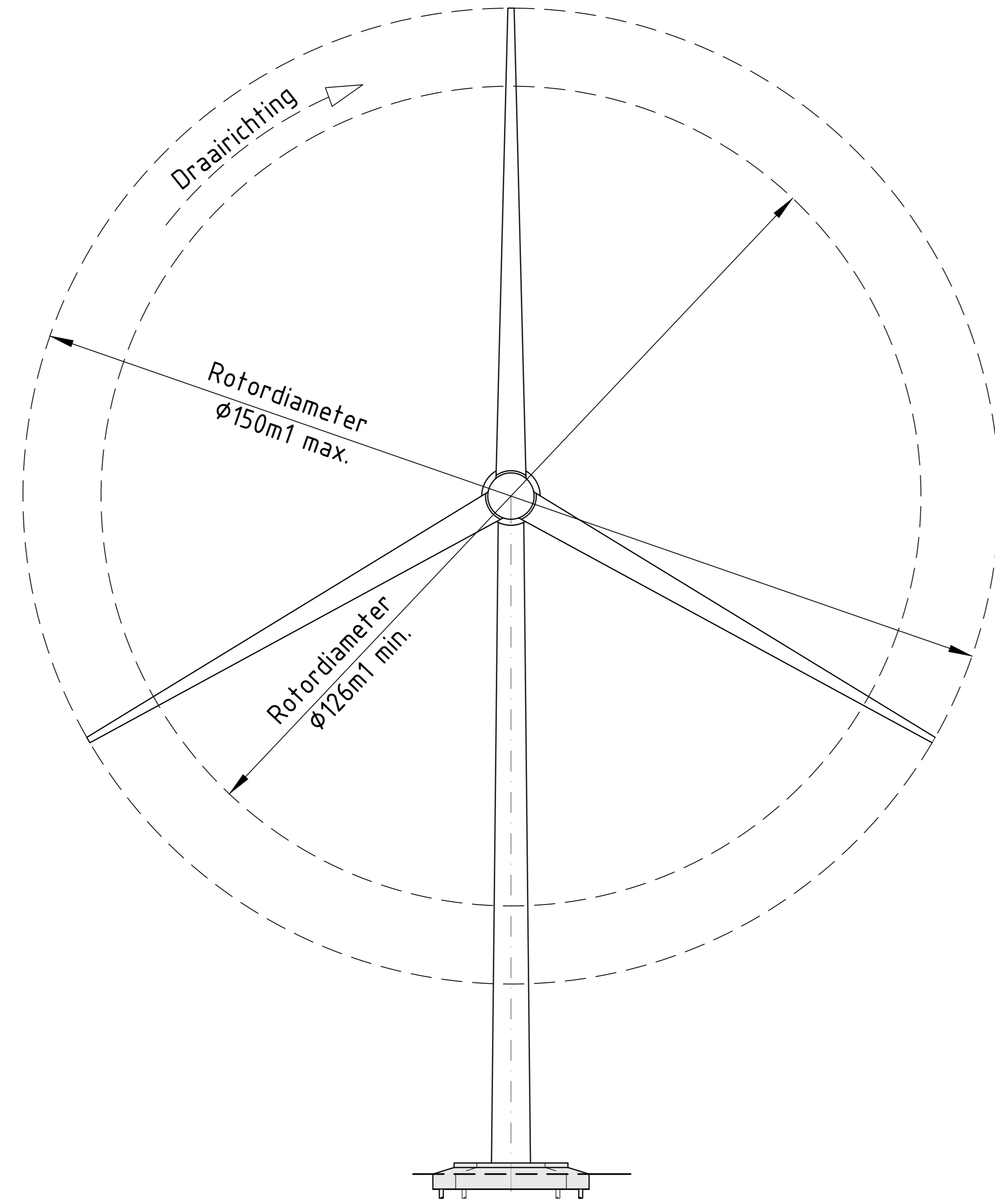
Windturbine Landmanslust
